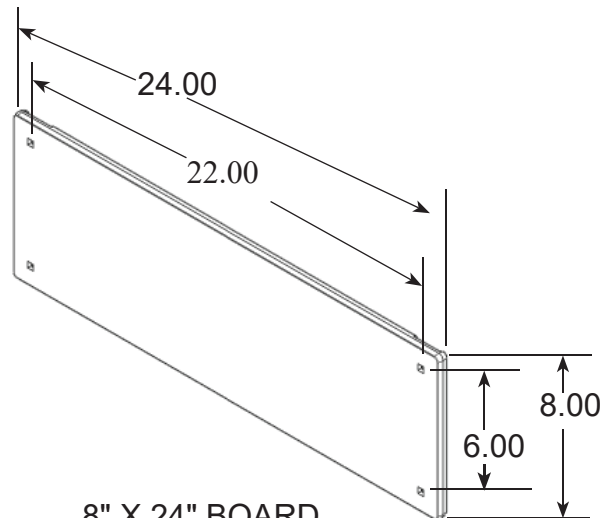
8" X 24" BOARD
